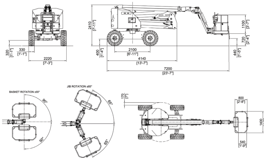
AJR18 ELC - WITH FIXED JIB - BASKET 2400 mm WORKING DIAGRAMS - TRAVELLING ALWAYS PERMITTED
