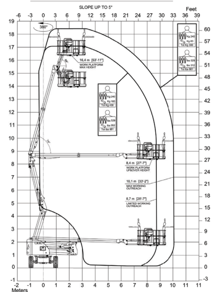
AJR18 ELC - WITH ROTATING JIB - BASKET 1400 mm WORKING DIAGRAMS - TRAVELLING ALWAYS PERMITTED
