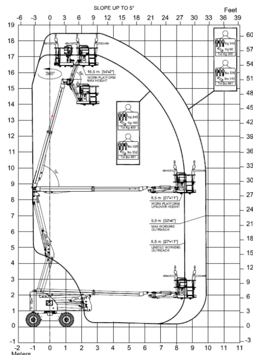
AJR18 ELC - WITH ROTATING JIB - BASKET 1400 mm WORKING DIAGRAMS - TRAVELLING ALWAYS PERMITTED
